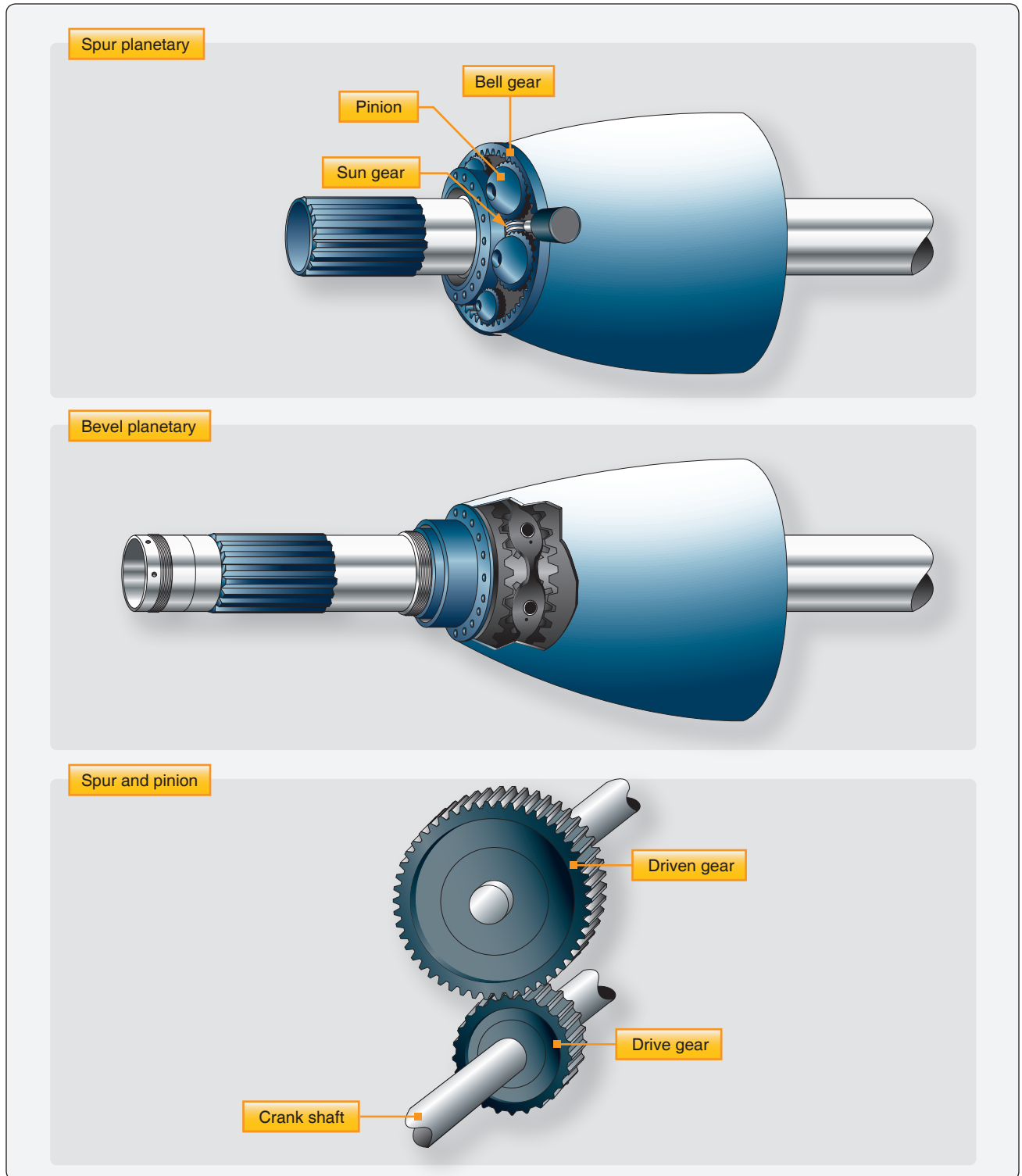
Figure 1-34. Reduction gears.
