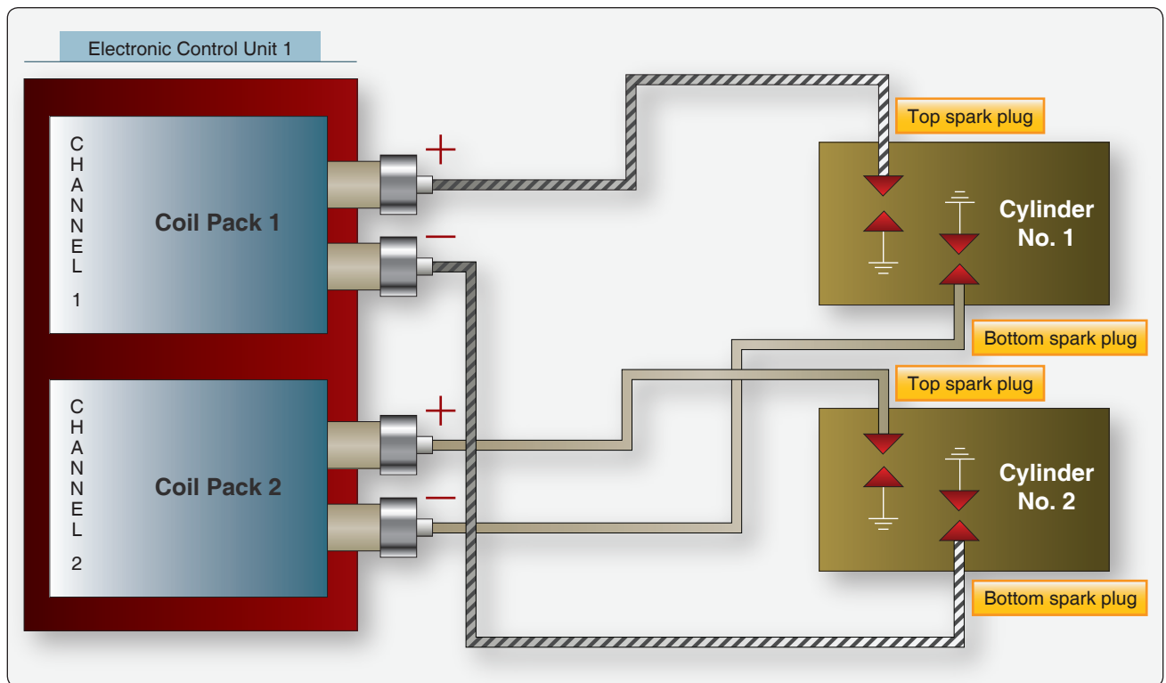
Figure 4-23. Ignition control.
