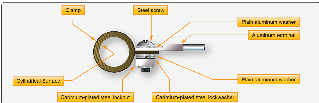
Figure 4-114. Bonding or grounding connections to a cylindrical structure.
