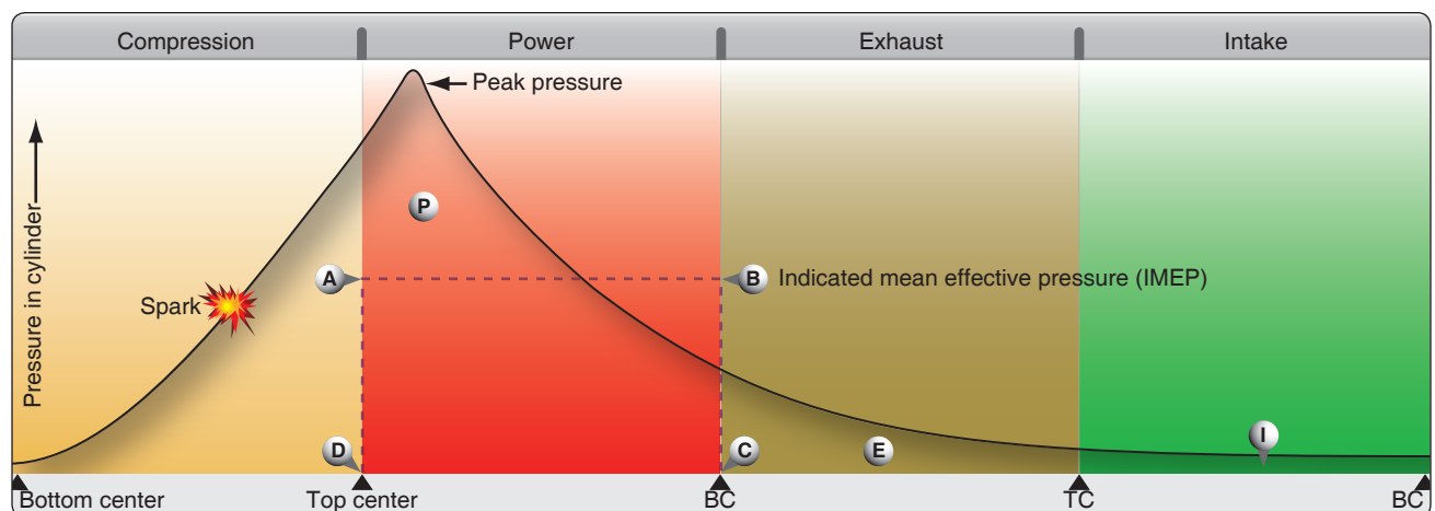
Figure 1-39. Compression ratio.
