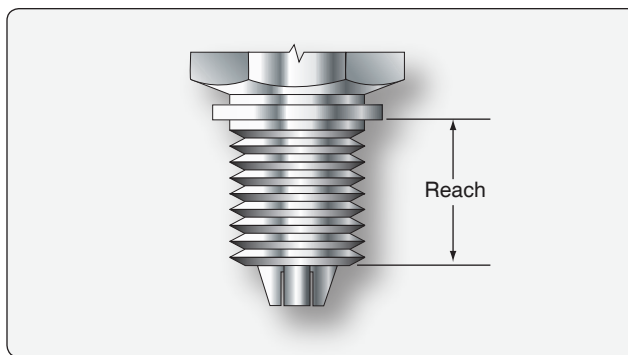
Figure 4-35. Spark plug reach.
