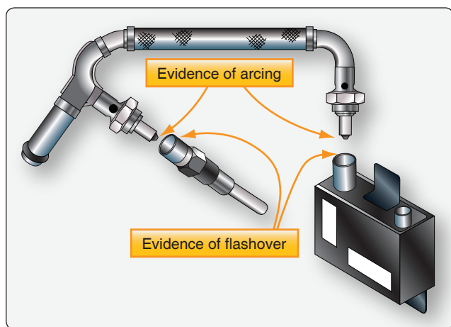
Figure 4-71. Flashover inspection.
