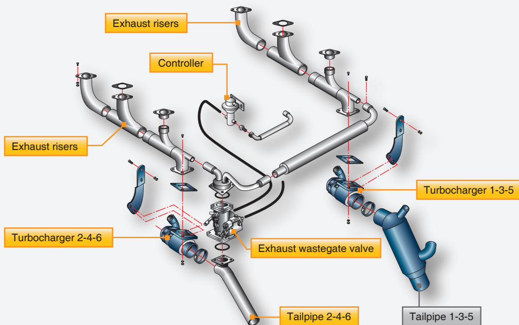
Figure 3-14. Exhaust gas turbine assembly.
