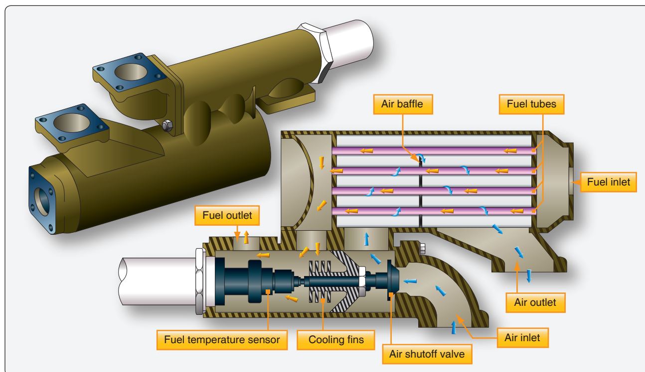
Figure 2-61. Fuel heater.
