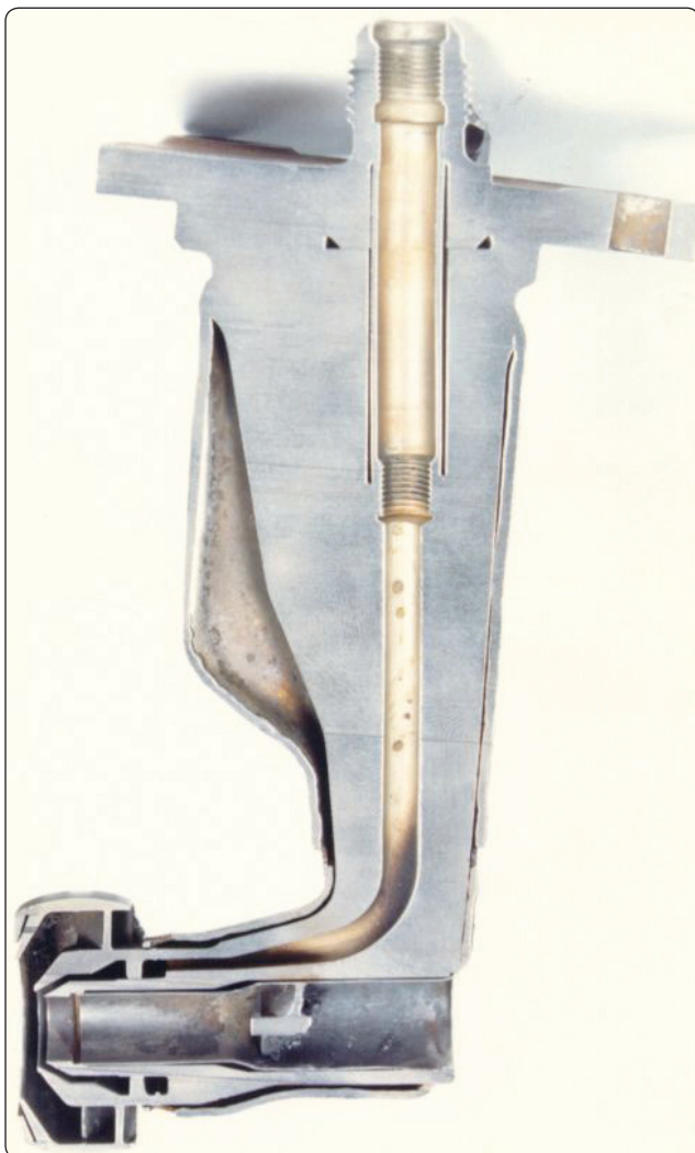
Figure 2-64. Simplex airblast nozzle cutaway.
