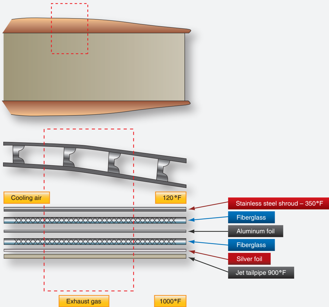
Figure 1-75. Insulation blanket with the temperatures obtained at the various locations shown.
