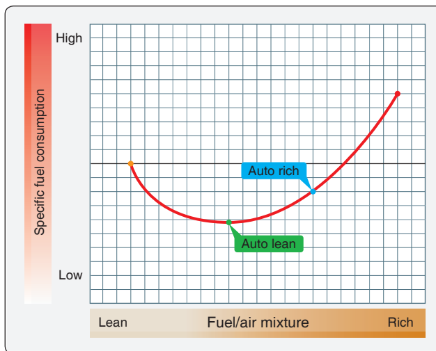
Figure 2-3. Specific fuel consumption curve.
