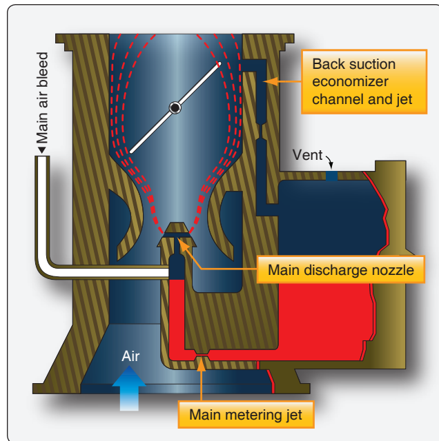
Figure 2-22. Float-type carburetor.
