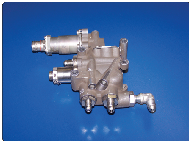
Figure 2-67. Flow divider.
