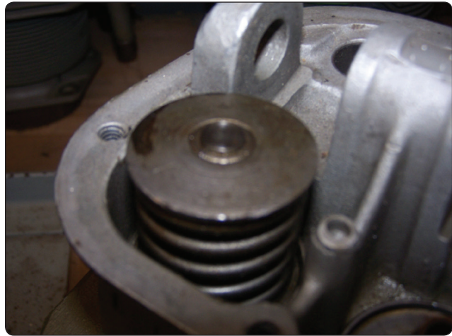
Figure 1-22. Stem keys forming a lock ring to hold valve spring retaining washers in place.
