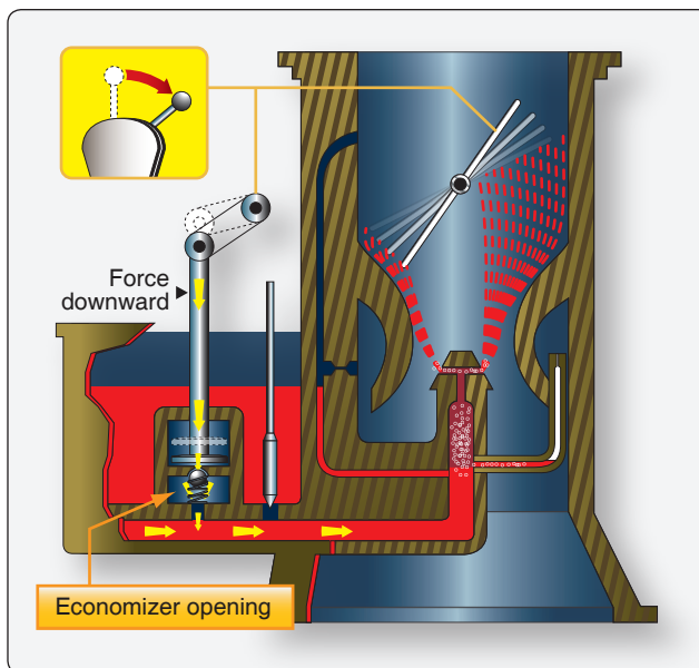
Figure 2-18. Accelerating system.
