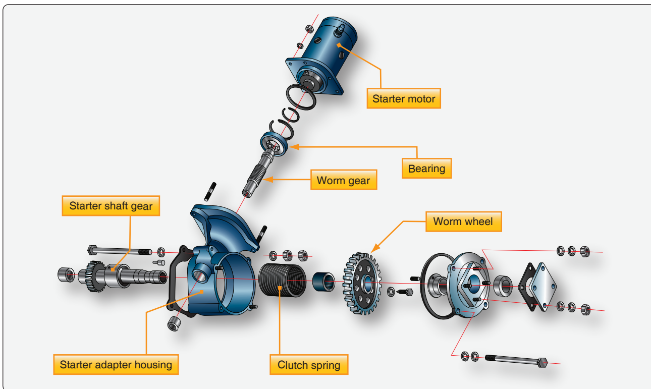
Figure 5-9. Starter adapter.
