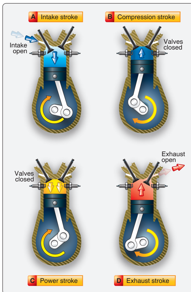
Figure 1-36. Four-stroke cycle.
