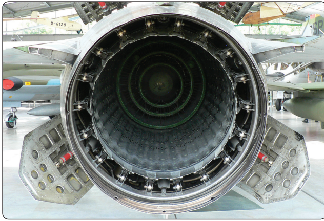
Figure 3-50. An example of a variable area exhaust nozzle used to increase or decrease exhaust flow during afterburn.
