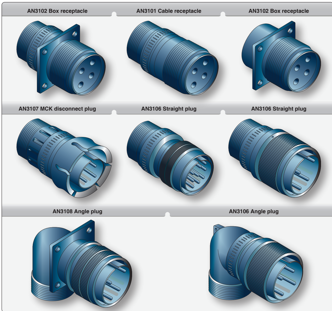
Figure 4-115. AN connectors.
