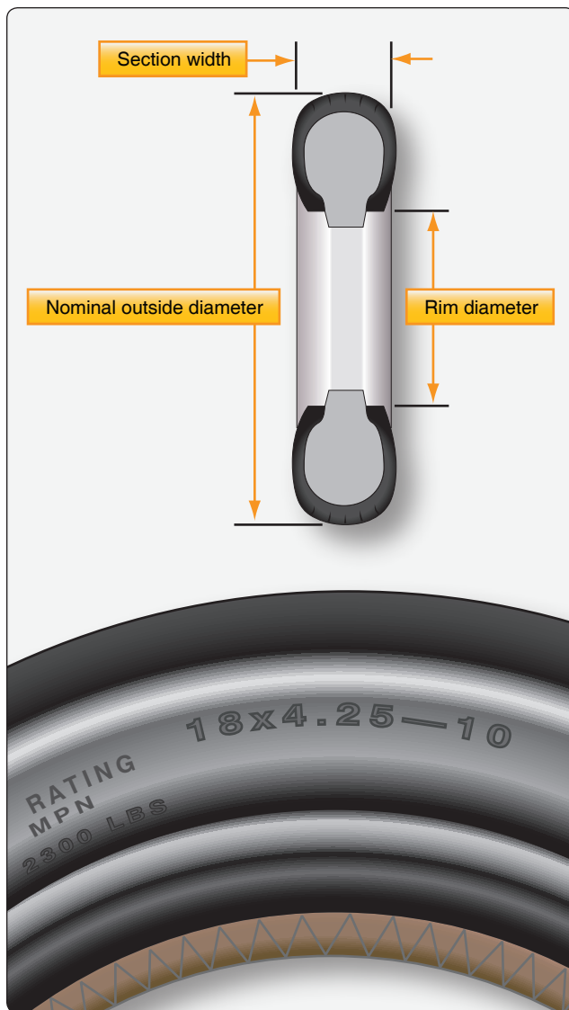
Figure 13-127. A Type VIII or three-part nomenclature tire is identified by 3 parameters: overall diameter, section width, and rim diameter. They are arranged in that order with the first two separated by an "X" and the second two separated by a "–." For example: 18 X 4.25—10 designates a tire that is 18 inches in diameter with a 4.25-inch section width to be mounted on a 10-inch wheel rim.
