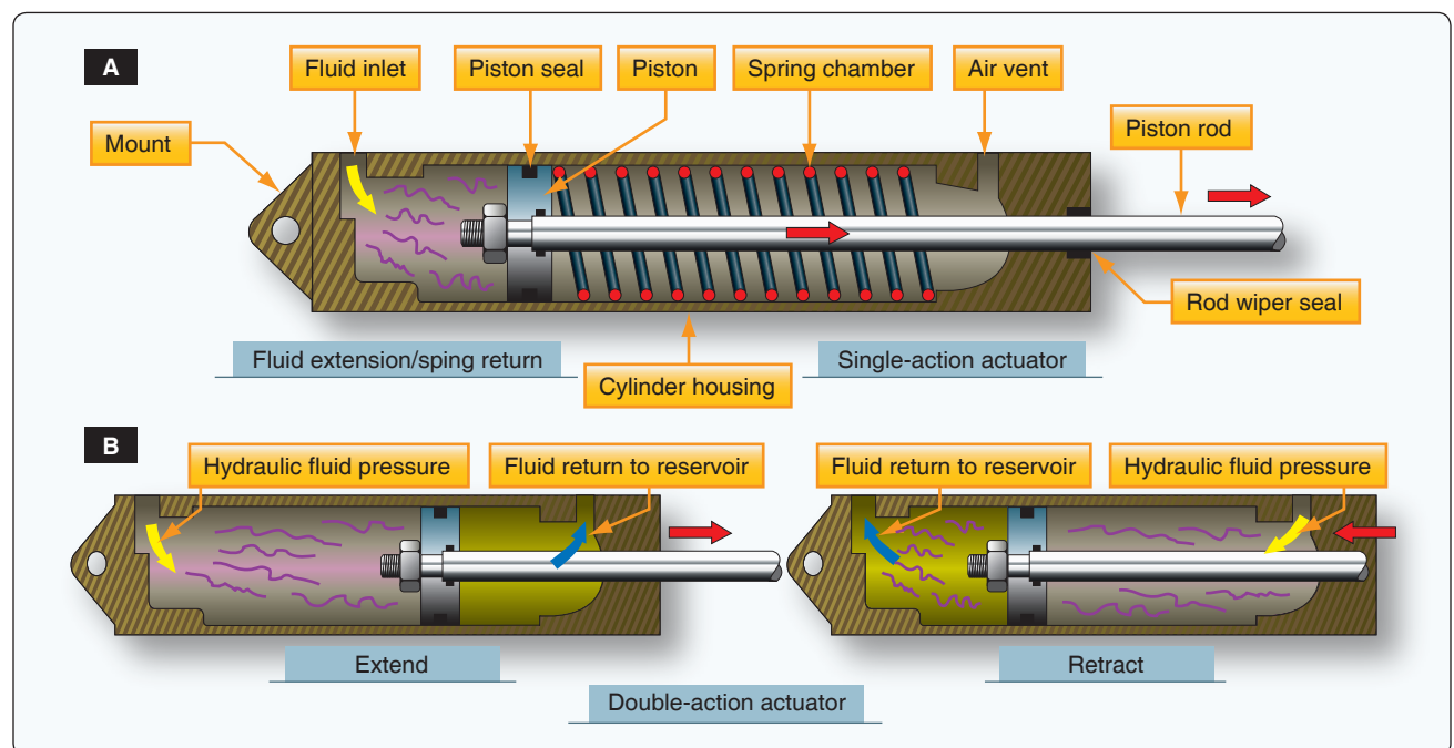
Figure 12-52. Linear actuator.
