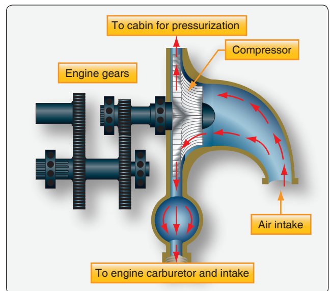
Figure 16-42. A reciprocating engine supercharger can be used as a source of pressurization if it is upstream of carburetion.
