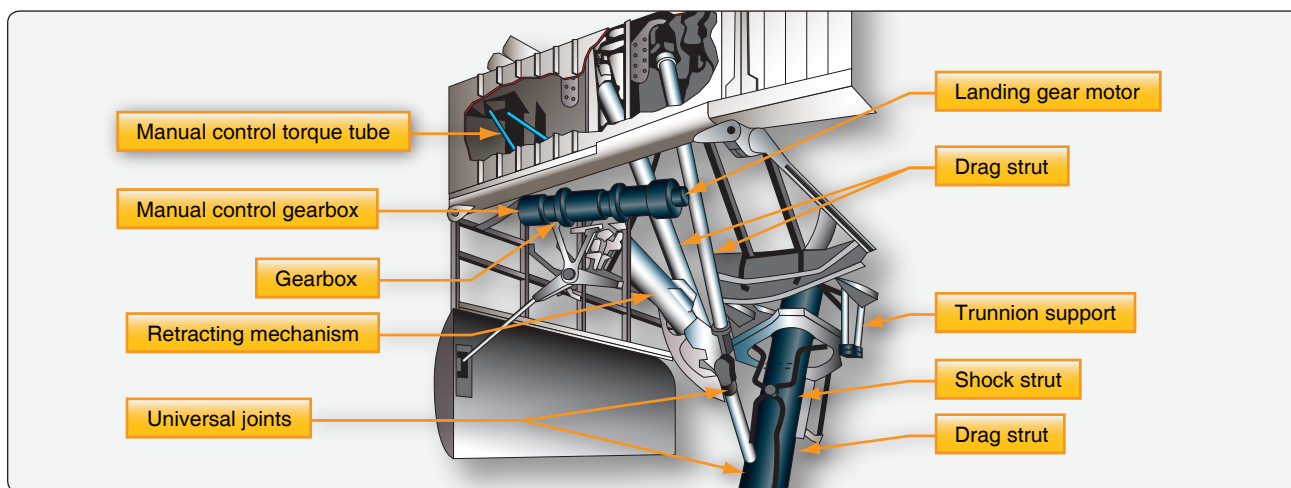
Figure 13-34. A geared electric motor landing gear retraction system.
